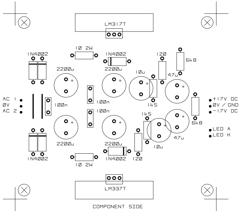
VI.1 CENTRE TAPPED TRANSFORMER VERSION
