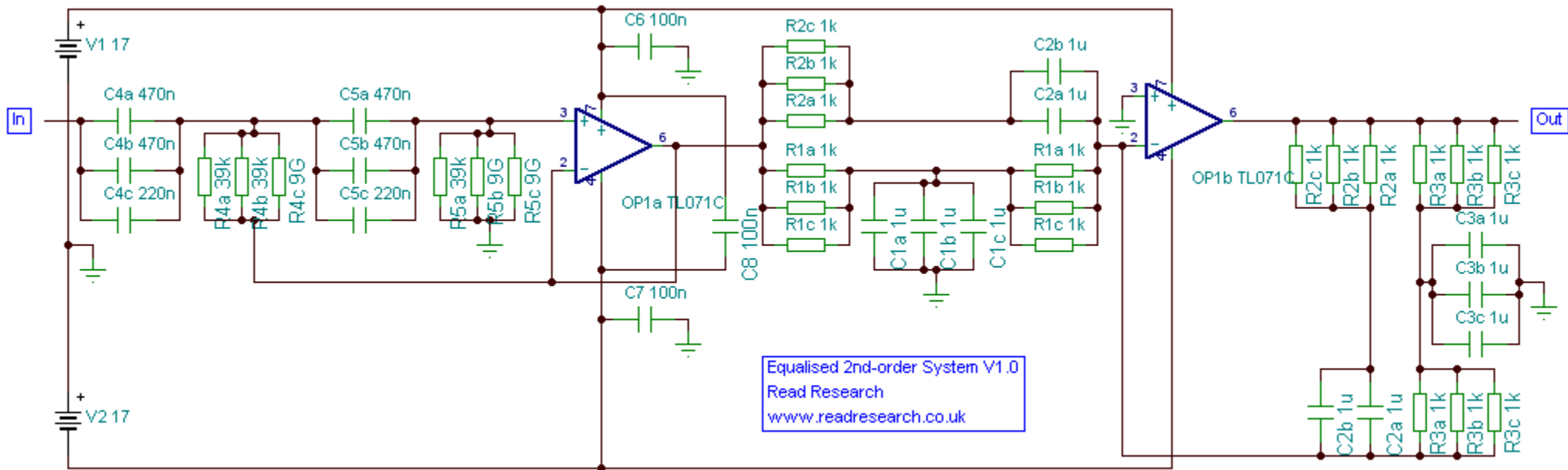
5 Hz Butterworth High-Pass Filter
